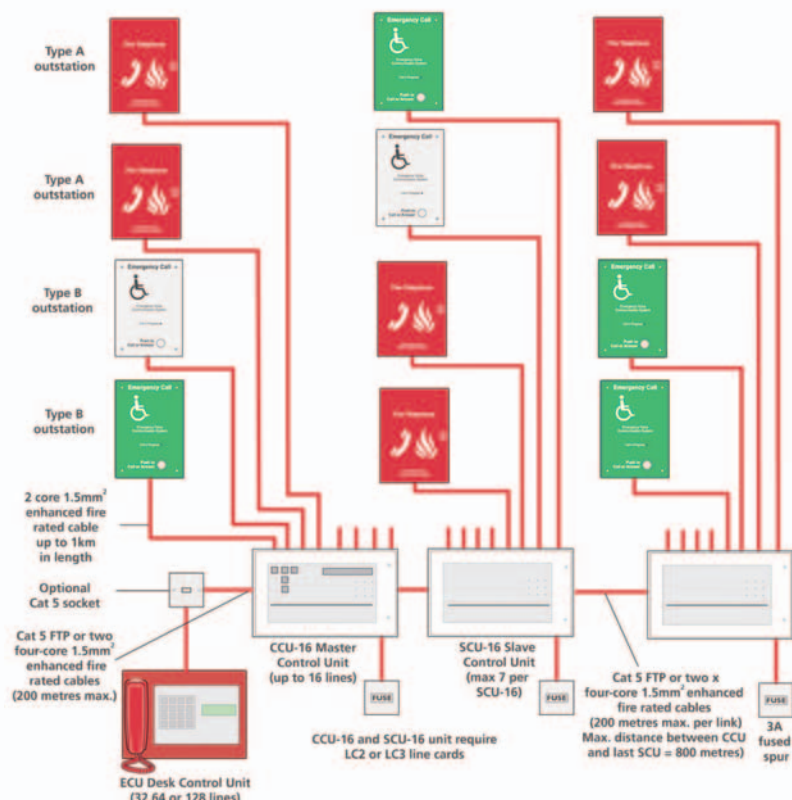
A typical SigTEL 16-128 Line system
